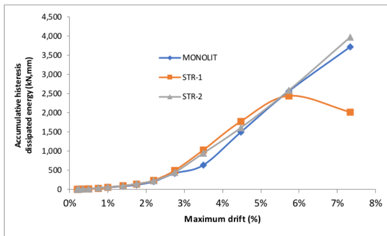
Fig. 7. Energy dissipation fungsi drift ratio
