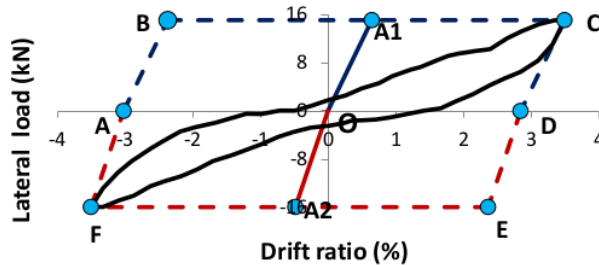
Fig. 2. Ideal energy dissipation
