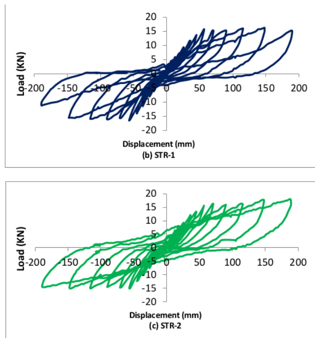
Fig. 5. Load displacement hysteretic curve
